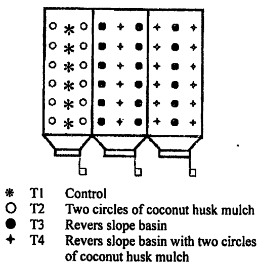
Fig. 1. Schematic diagram of experimental layout within run-off plots
