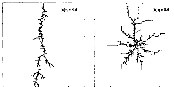
Figure 6: Simulated lightning and surface discharge patterns with fractal dimensions comparable to the experimentally measured observations
