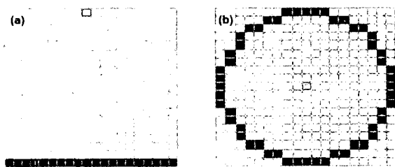
Figure 1: Initial charge configuration; black: \phi=1 grey: \phi=0 (a) Lightning discharge (b) Surface discharge
