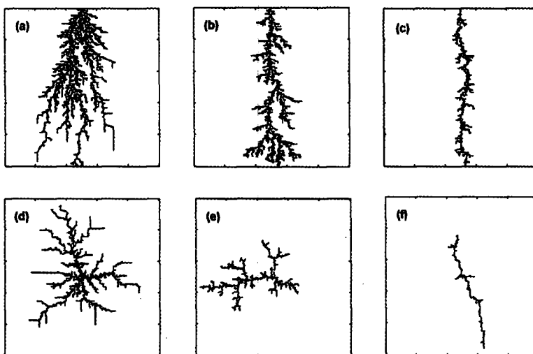
Figure 4: Simulated lightning discharge patterns when (a) \eta=0.5 , (b) \eta=1 and (c) \eta=1.5 , and, surface discharge patterns when (d) \eta=1 , (e) \eta=2 and (f) \eta=4
