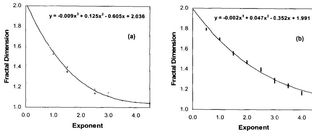
Figure 5: Variation of fractal dimension with \eta (a) Lightning discharges (b) Surface discharges
