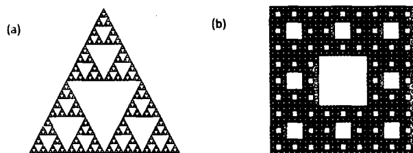
Figure 2: Fractal shapes used in testing the implemented algorithms (a) Sierpinski Gasket (b) Sierpinski Carpet
