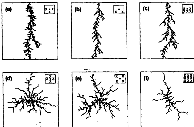
Figure 3: Simulated lightning and surface discharge growth patterns for \eta=1 with the insets showing the cell configurations
